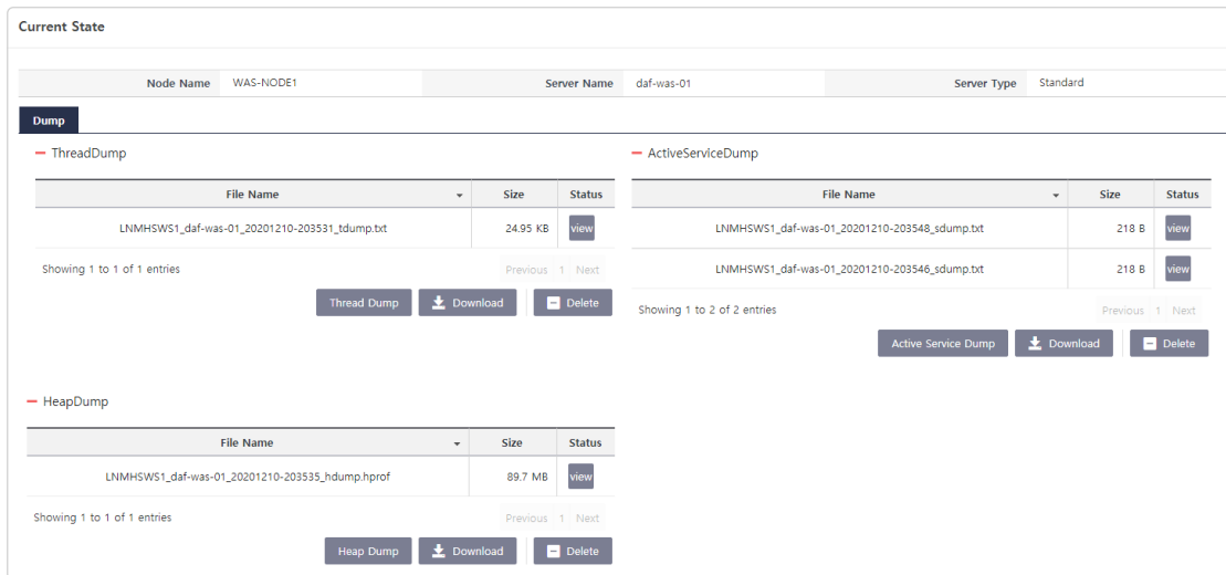
Figure 24. Dump 창
