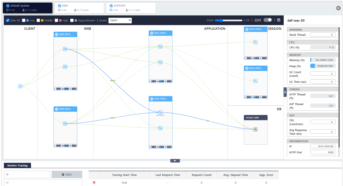
Figure 66. Topology 화면
