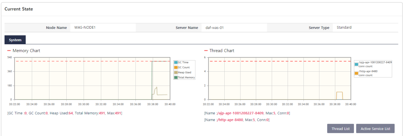
Figure 25. System 탭
