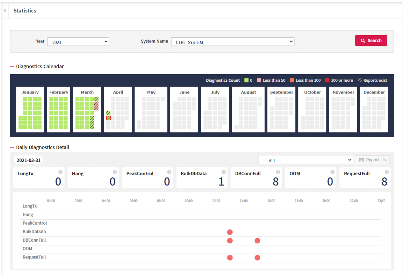
Figure 32. Statistics 화면
