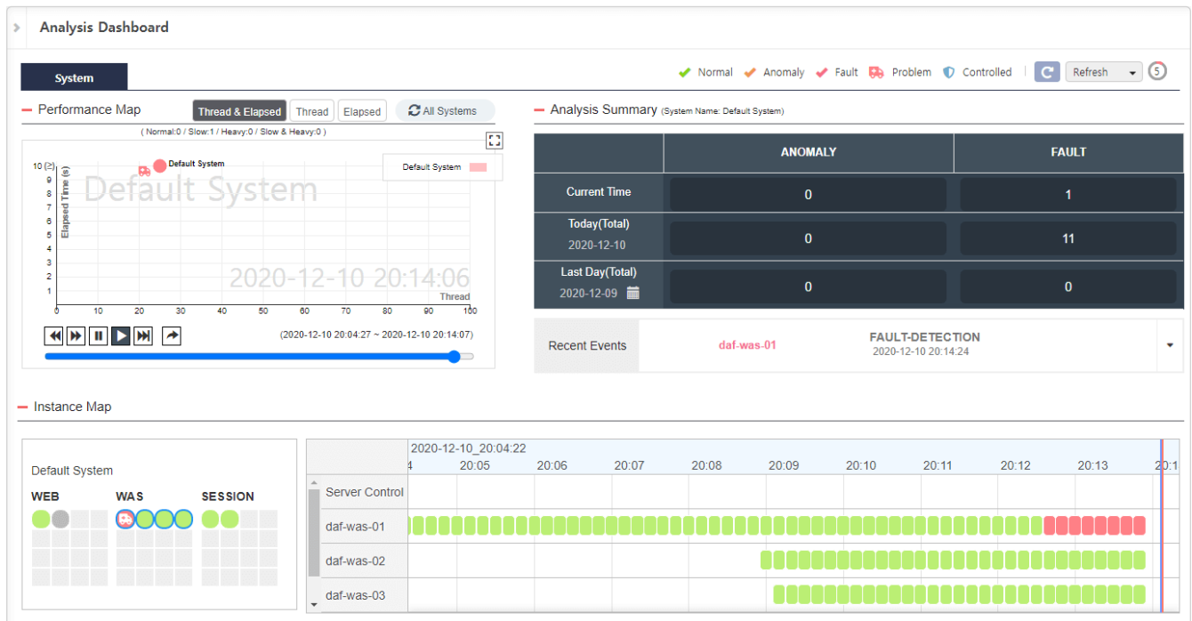
Figure 27. Analysis Dashboard
