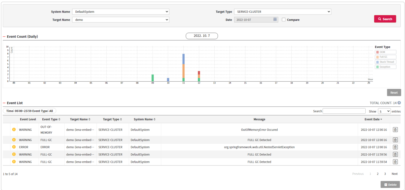
Figure 30. Event Dashboard
