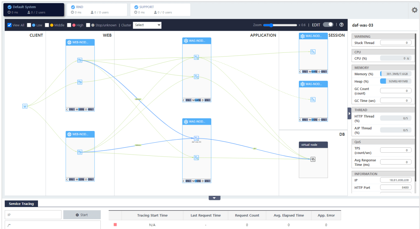
Figure 87. Topology 화면
