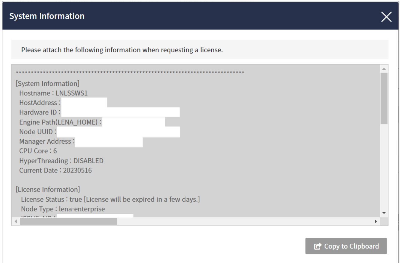
Figure 93. System Information
