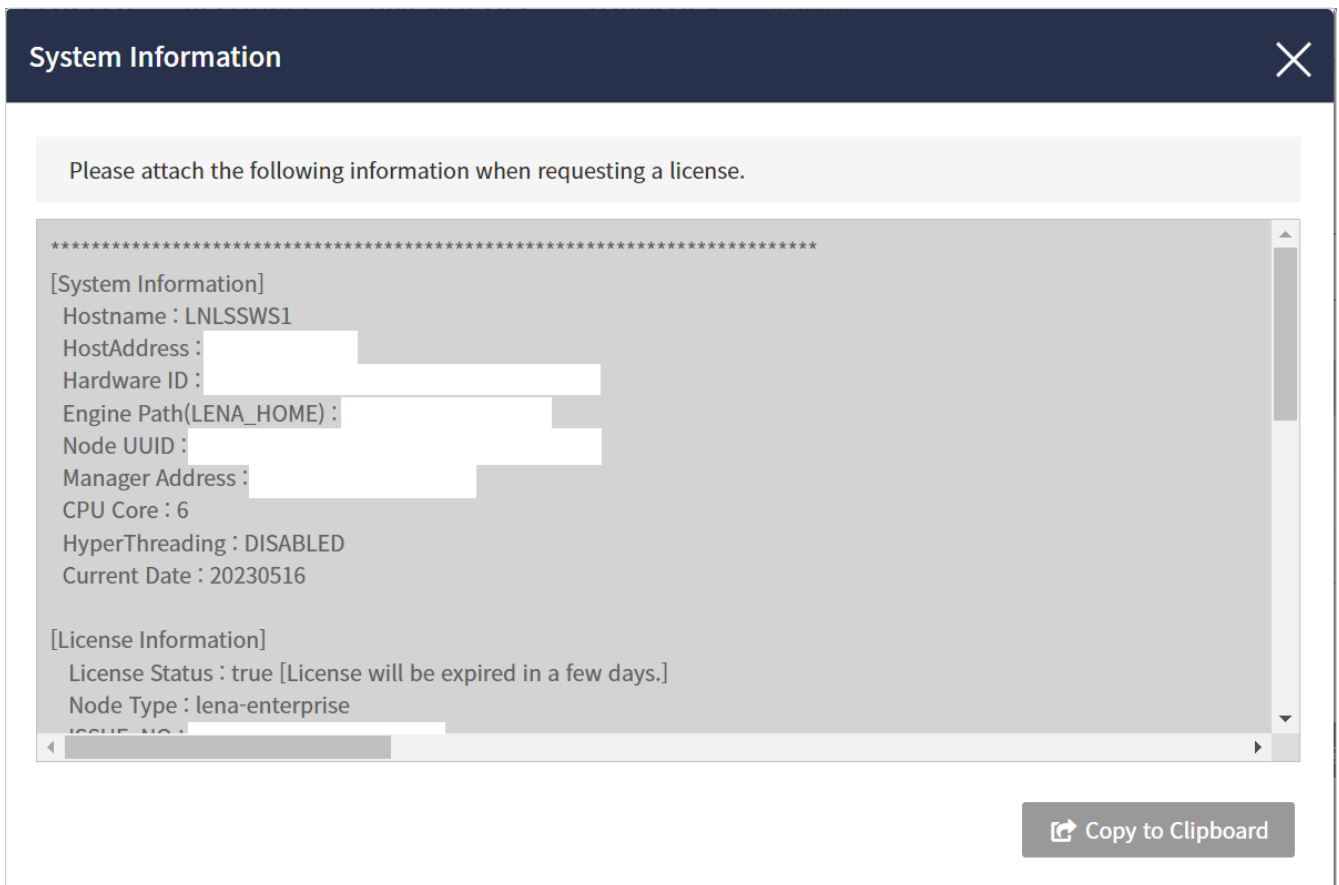
Figure 95. System Information
