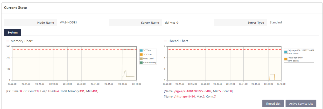
Figure 59. System 탭
