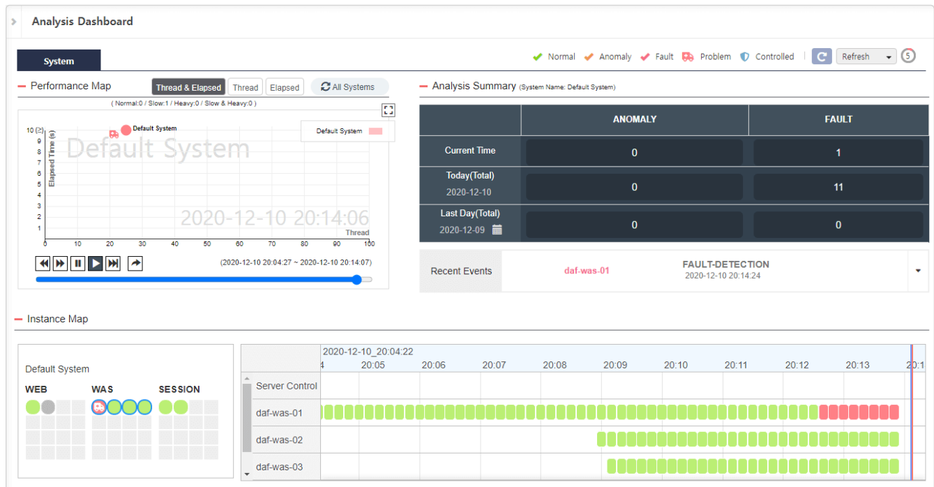
Figure 61. Analysis Dashboard
