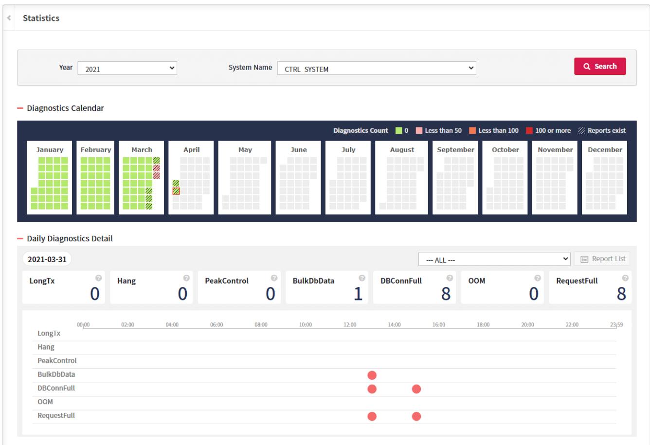
Figure 66. Statistics 화면
