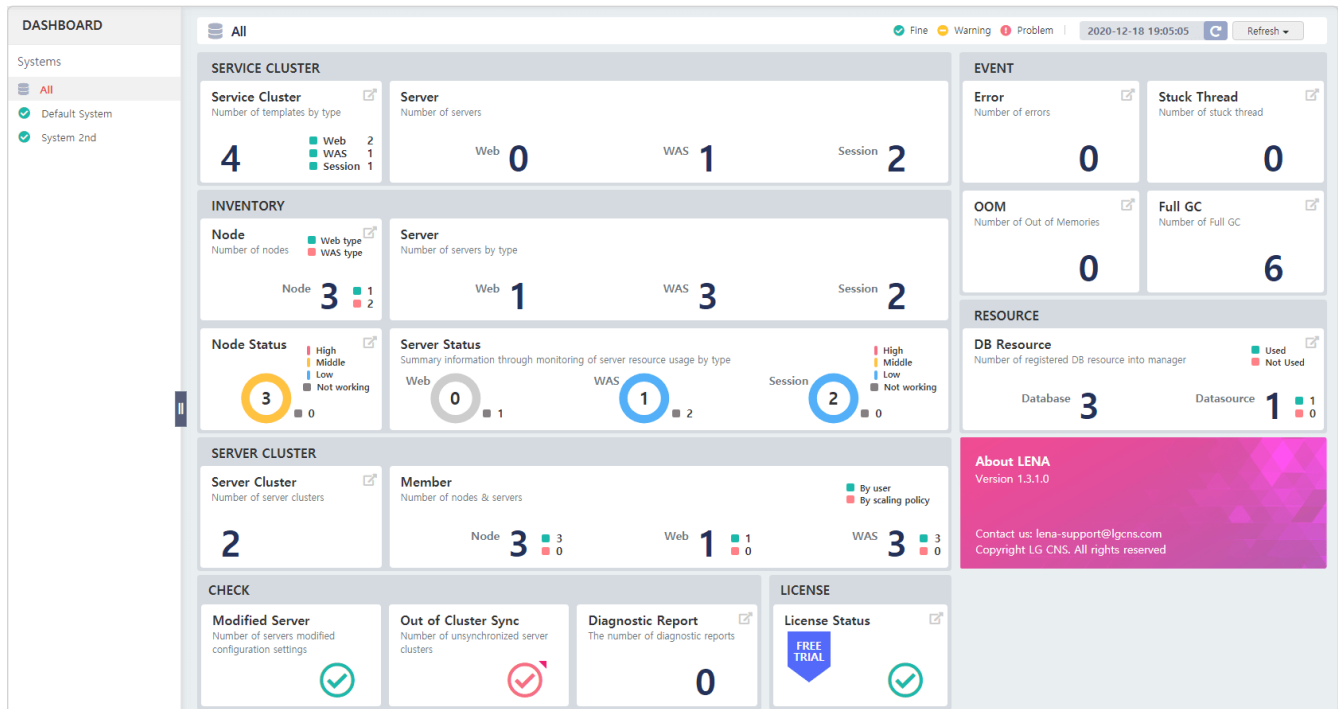
Figure 3. Dashboard
