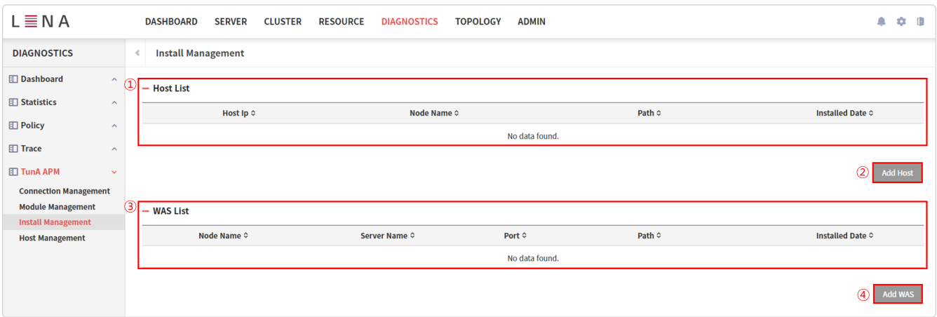
Figure 56. Install Management 화면
