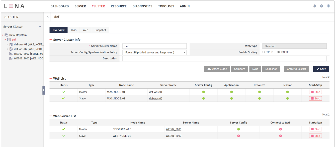
Figure 8. Server Cluster 화면
