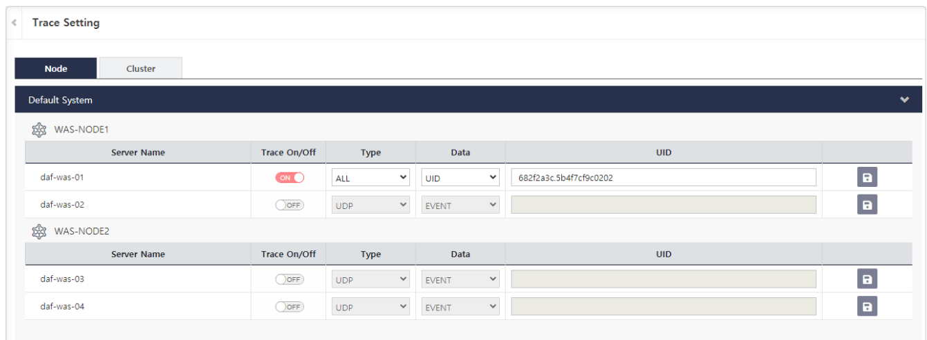
Figure 82. Trace Setting 화면
