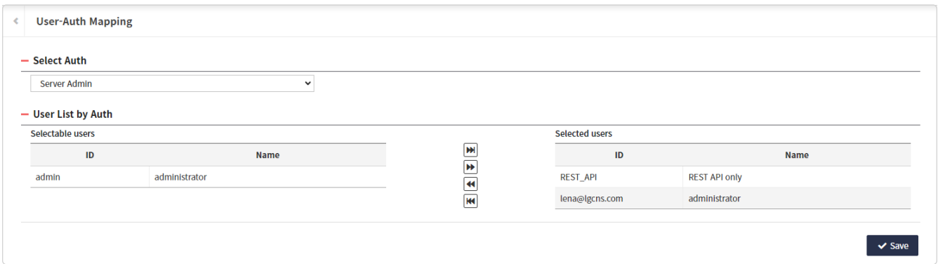
Figure 88. User-Auth Mapping 화면
