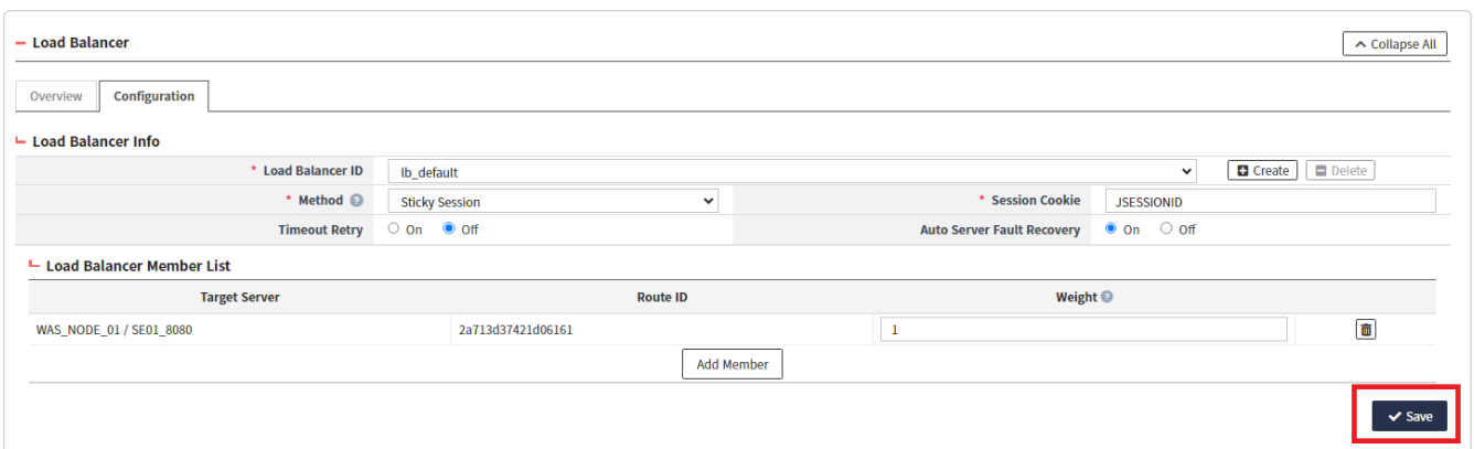
Figure 27. 연동한 WAS 목록 저장
