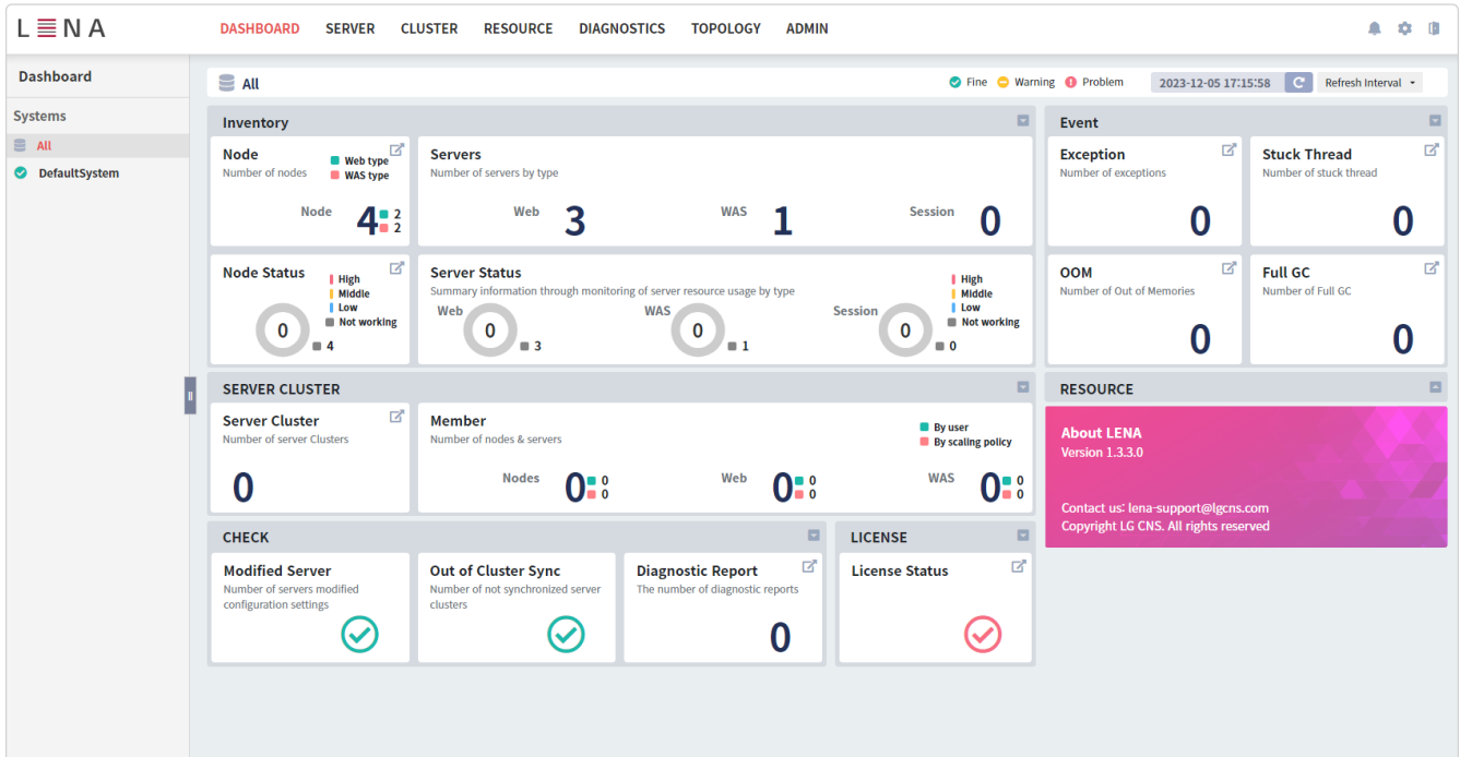
Figure 3. Dashboard
