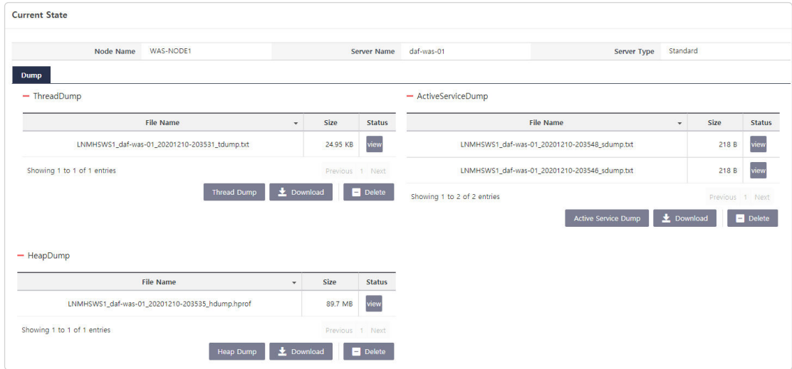
Figure 55. Dump 창
