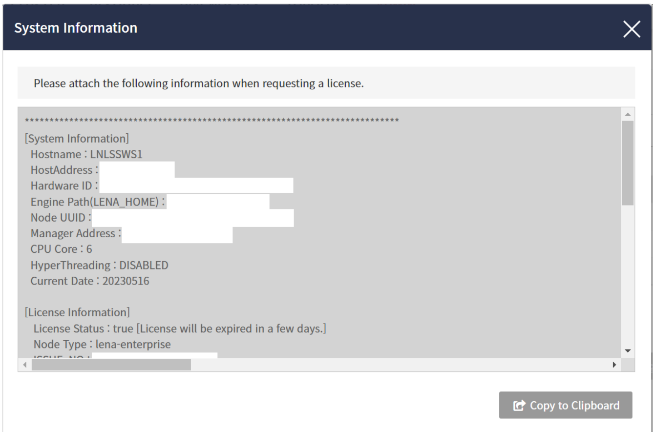
Figure 85. System Information
