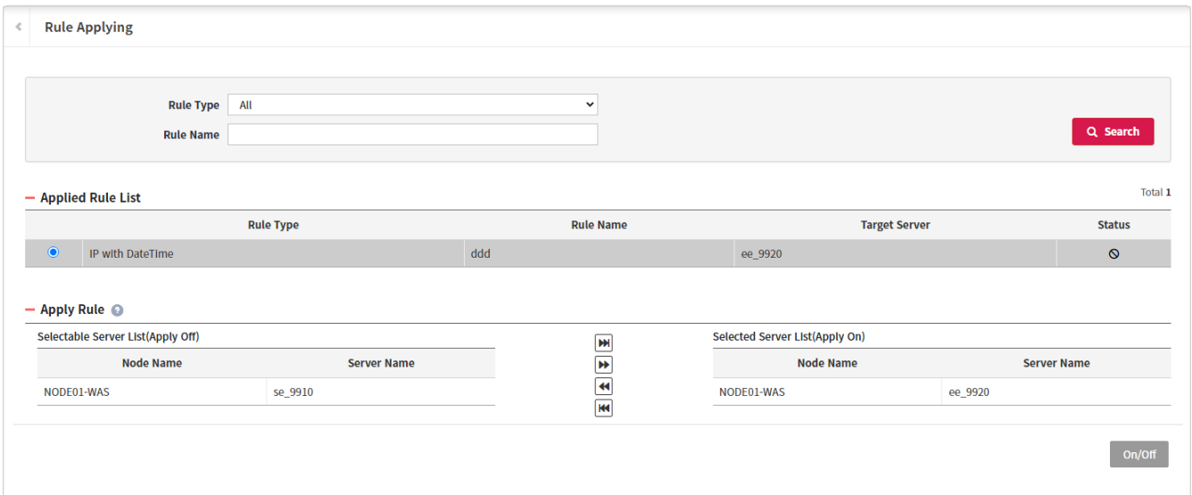
Figure 90. Rule Applying 화면
