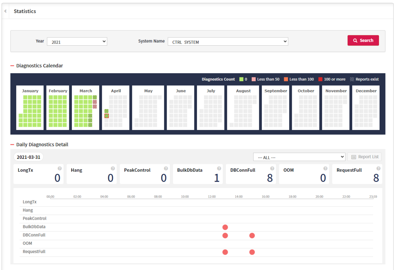
Figure 62. Statistics 화면
