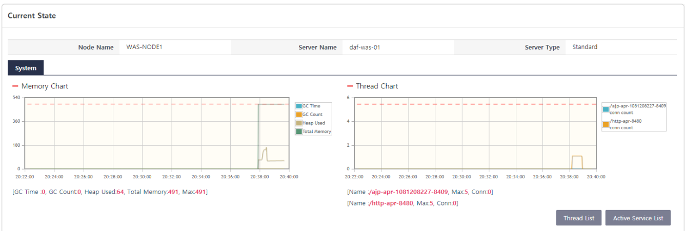
Figure 55. System 탭
