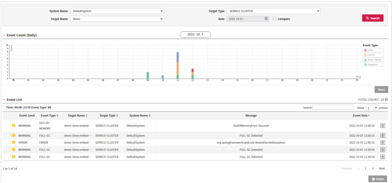
Figure 60. Event Dashboard
