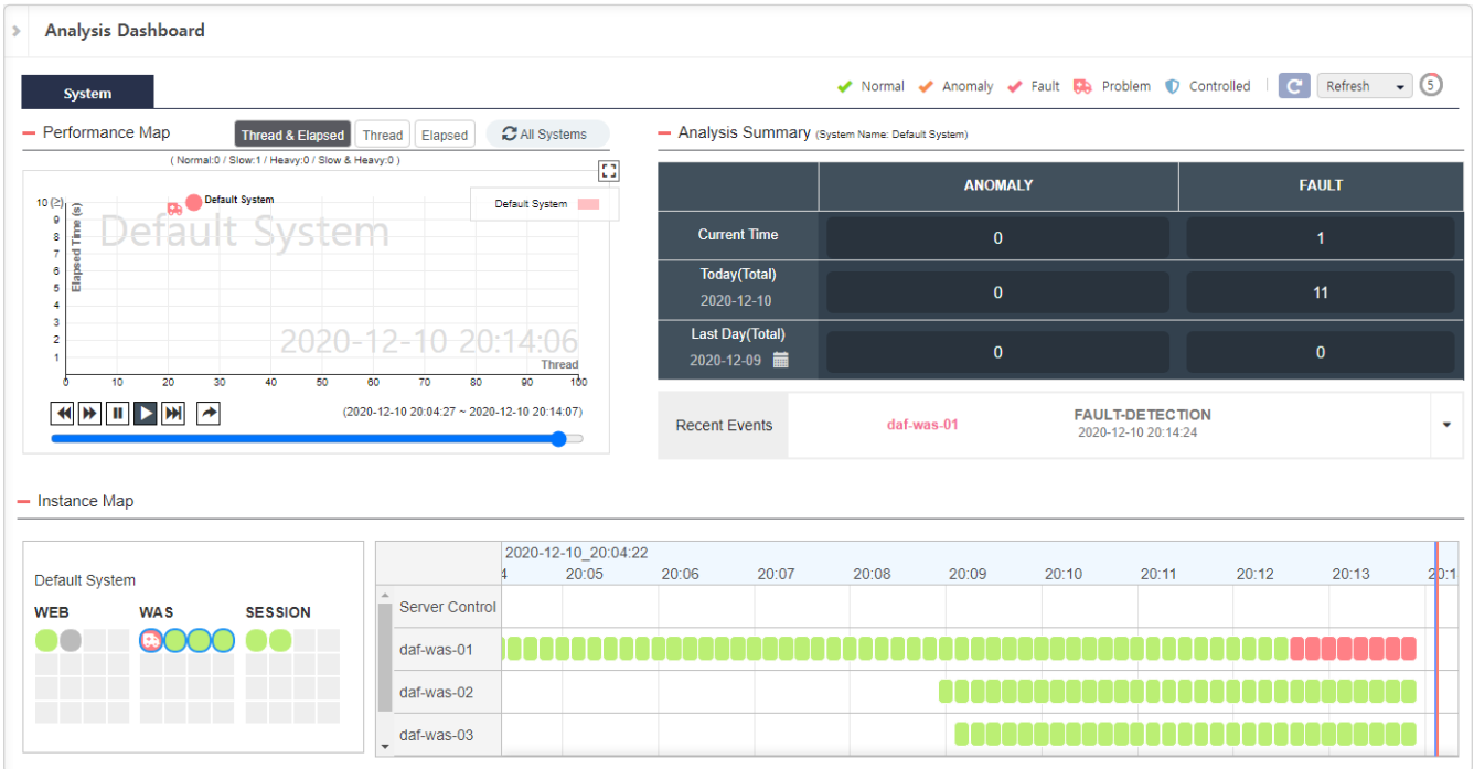
Figure 57. Analysis Dashboard
