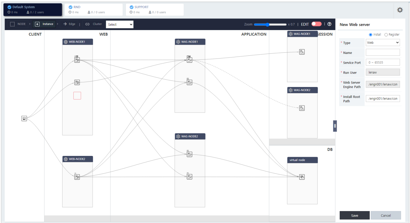
Figure 76. Topology Control [Edit: ON]
