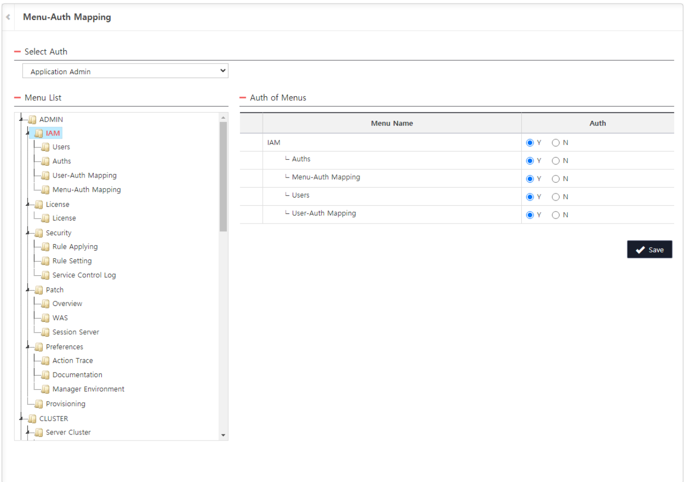
Figure 80. Menu-Auth Mapping 화면
