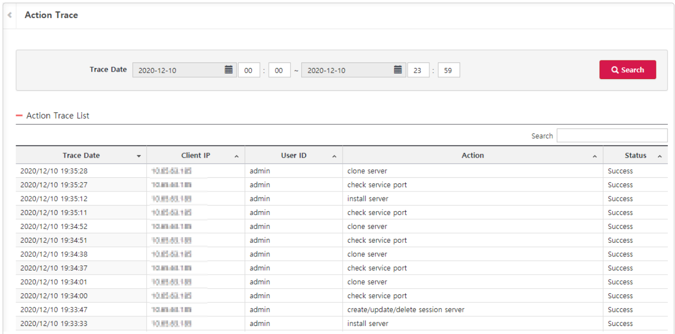
Figure 91. Action Trace 화면
