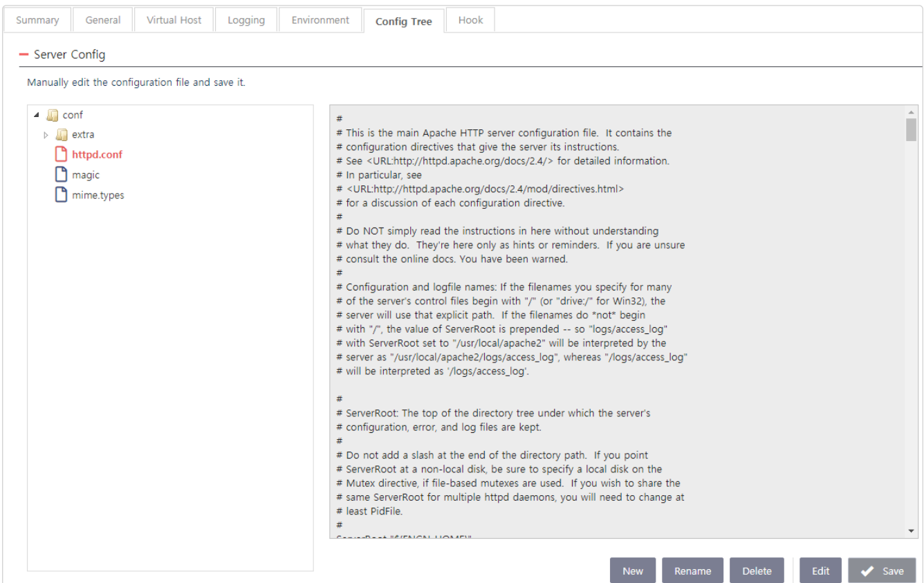
Figure 38. Web Server Template Config Tree 탭
