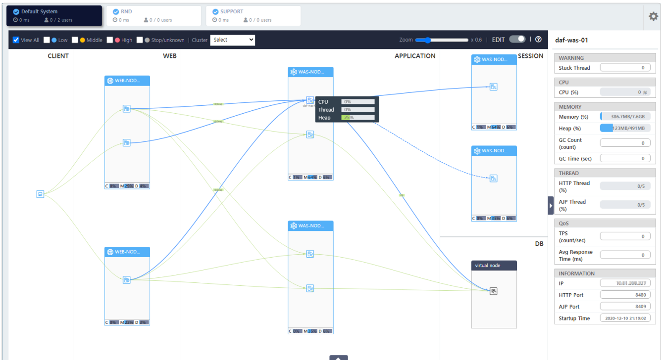
Figure 75. Topology Control [Edit: OFF]
